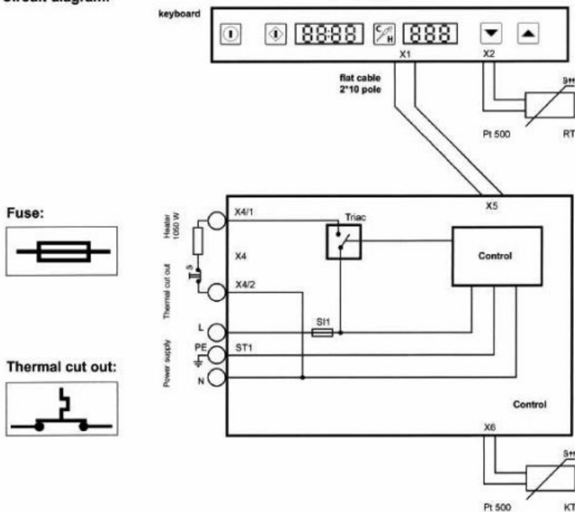
Circuit diagram:
